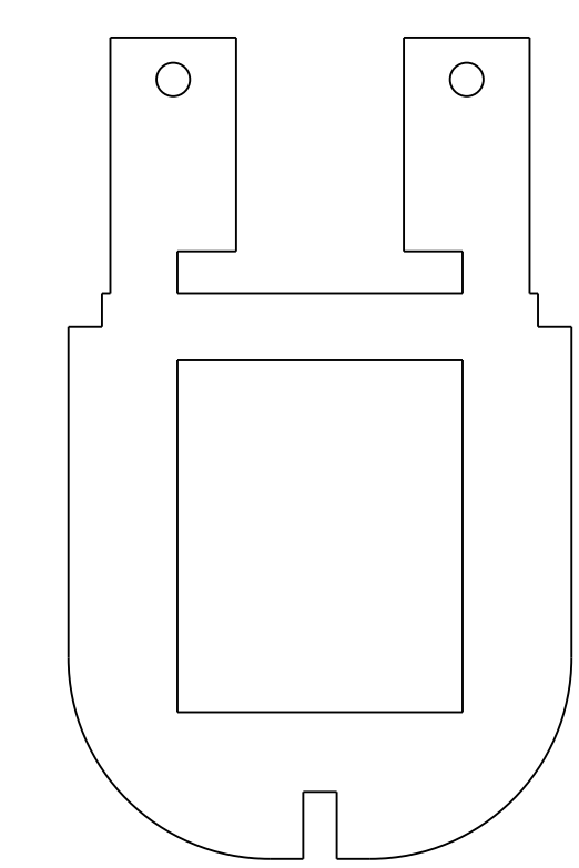
Spant 14
